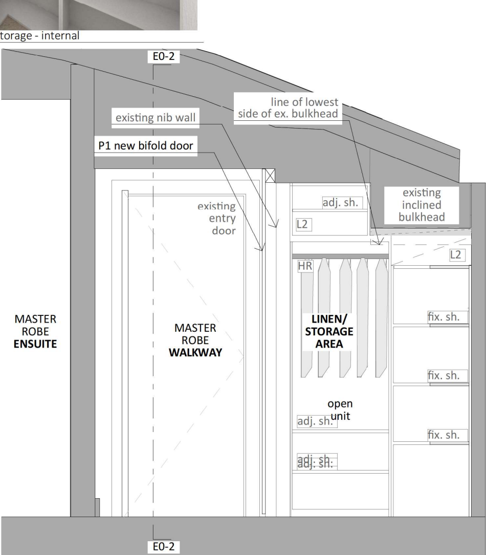
S-02 Linen Storage Section 1:25
