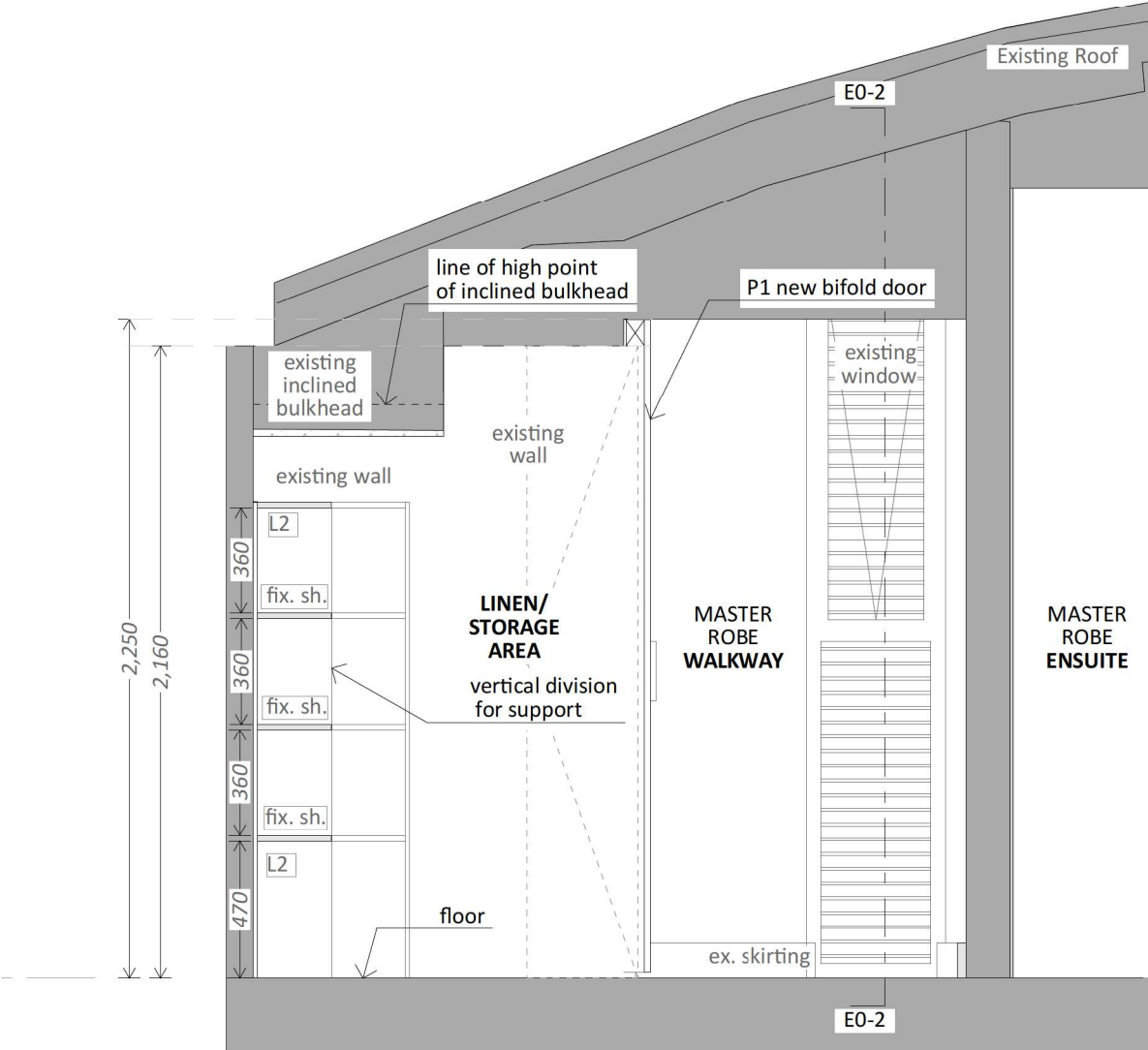
S-01 Linen Storage Section 1:25
